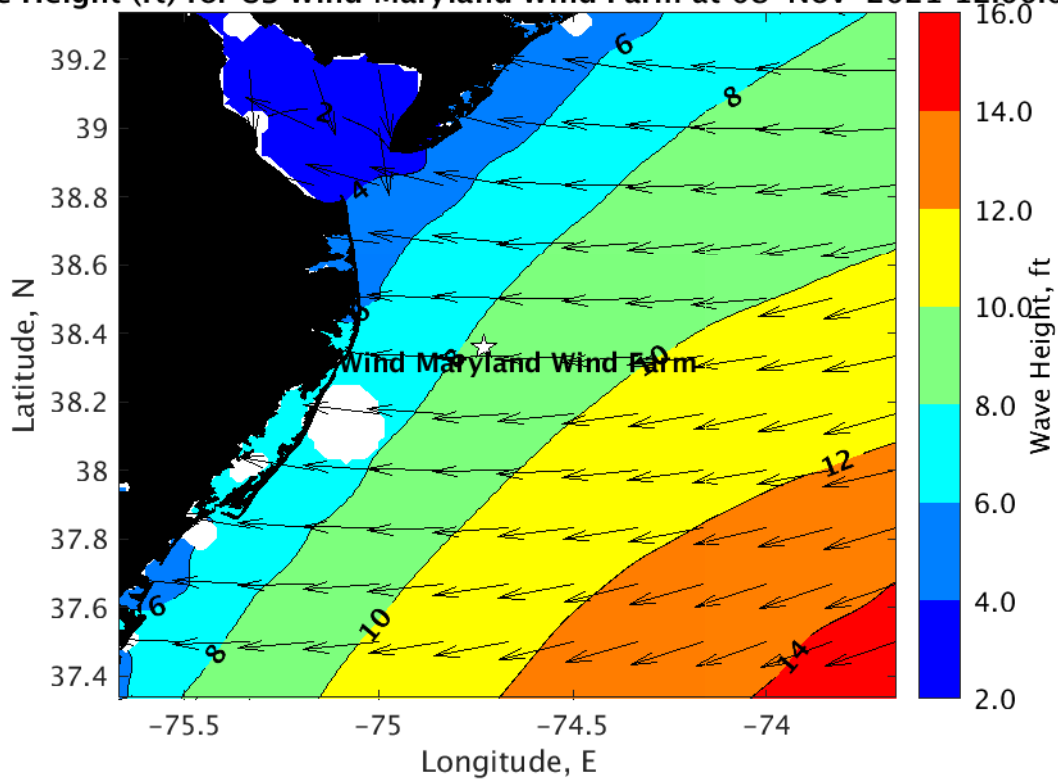
Wave Height (ft) for US Wind Maryland Wind Farm at 08-Nov-2021 12:00:00
